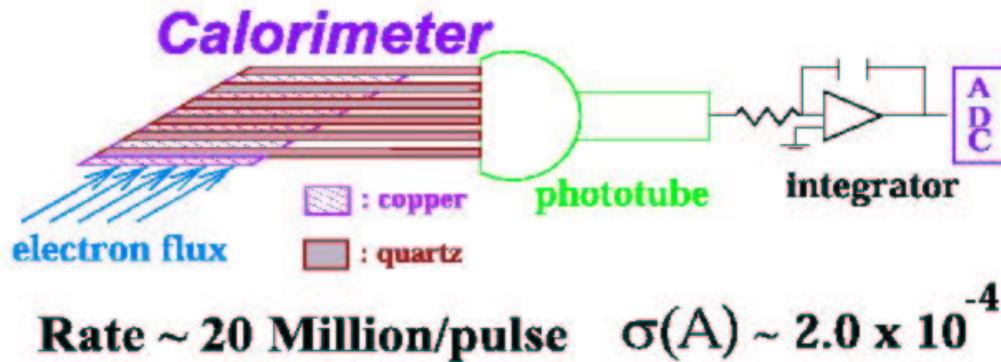
Figure 6. Cherenkov Detection
