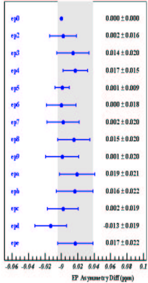
EP Asymmetry Diff vs cut, 48 GeV
