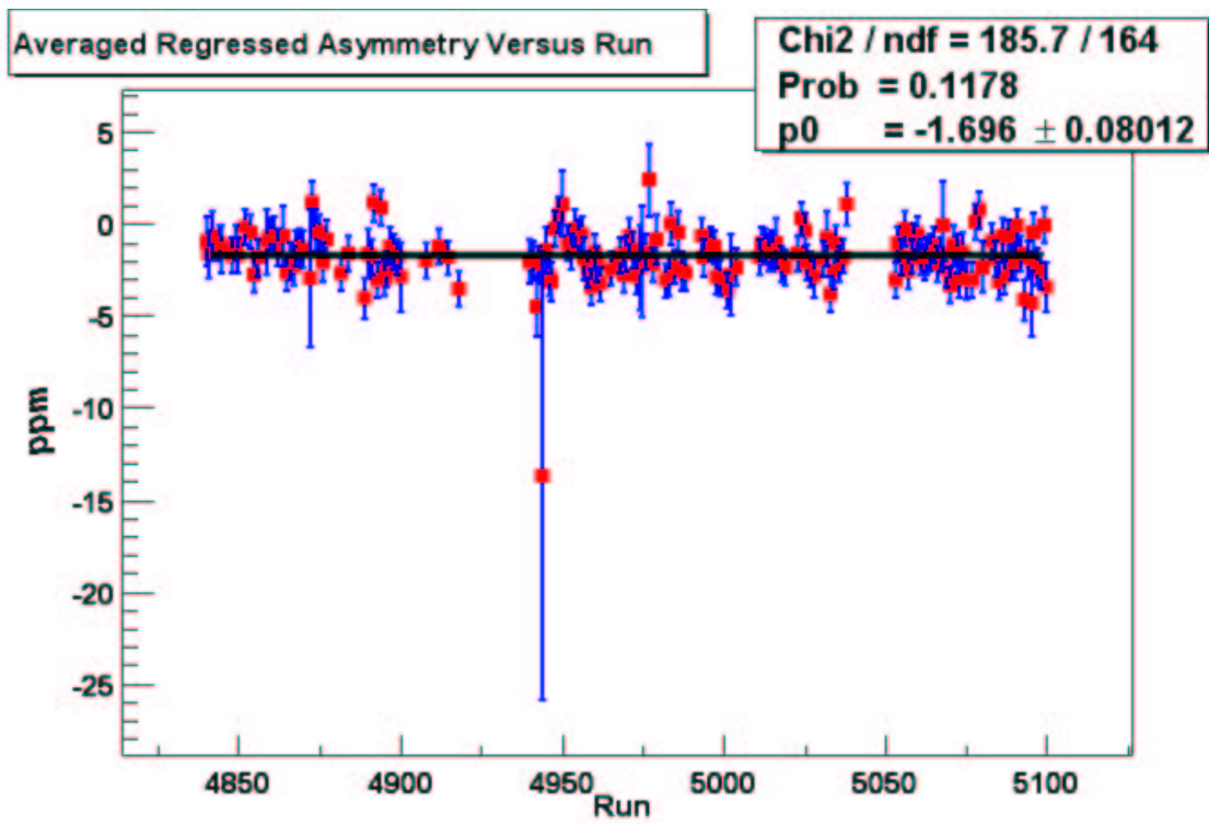
Figure 13. 48 GeV
