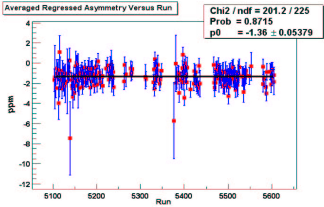
Figure 12. 45 GeV
