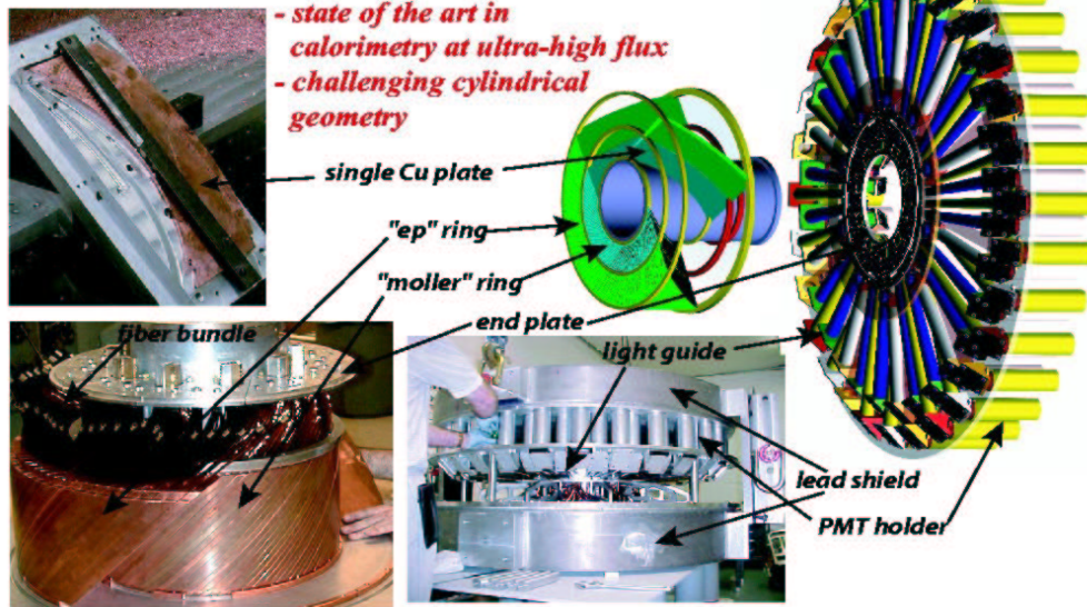
Figure 5. Schematic of the Detector
